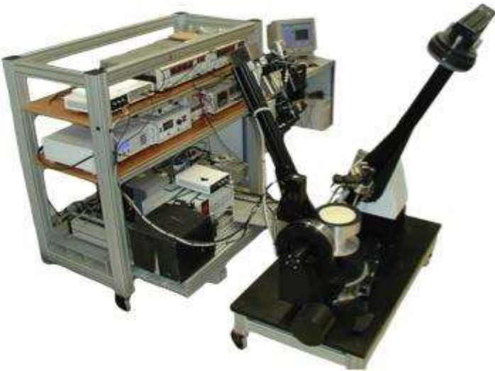
Spectro-Gonio Radiometer with its stabilized monochromatic source, the goniometer with illumination mirror, an open sample holder with sulfur powder and the detectors and the goniometer and detection electronics.
